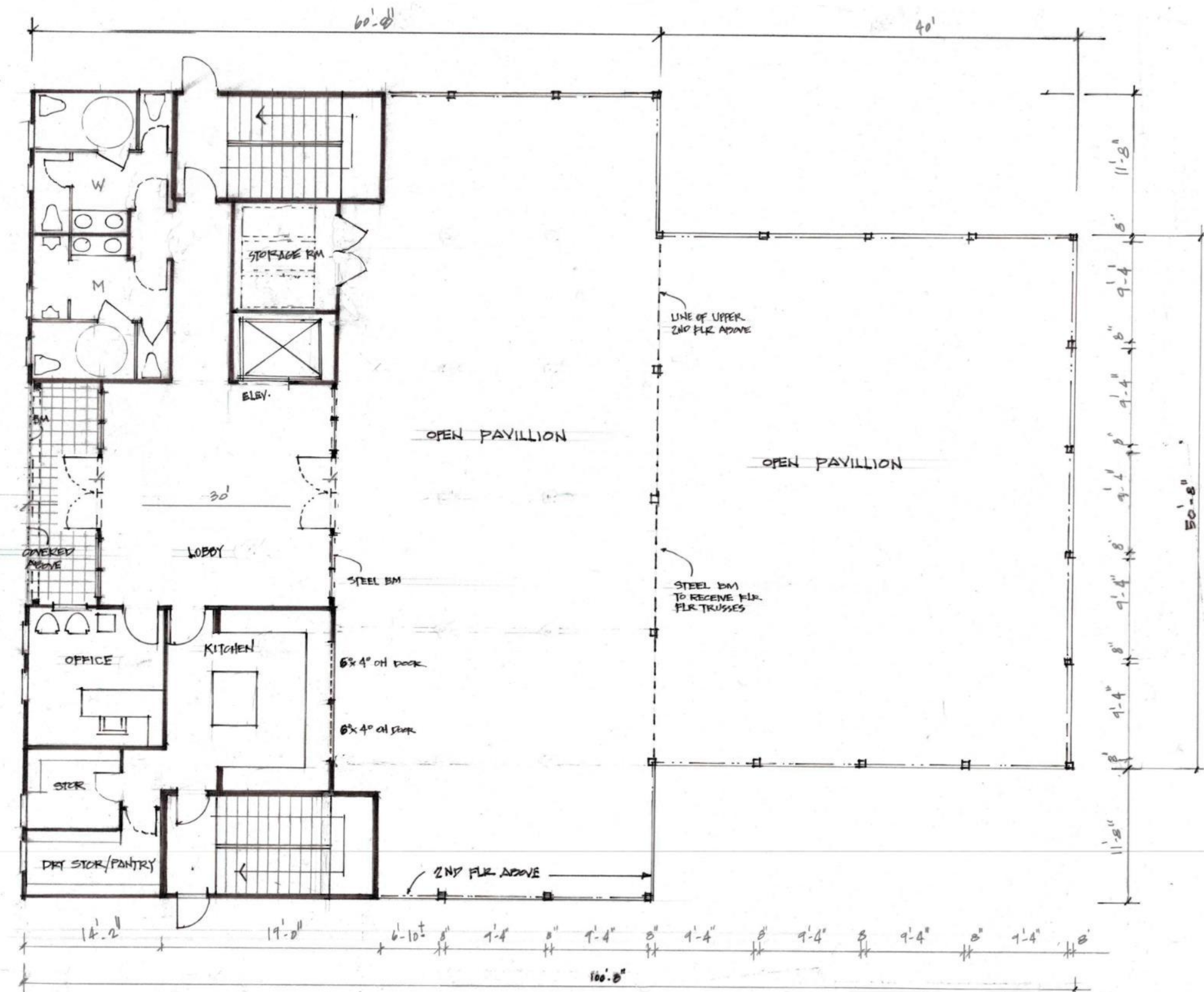
CONCEPT GROUND FLOOR PLAN - N.T.S. (NOT TO SCALE)
